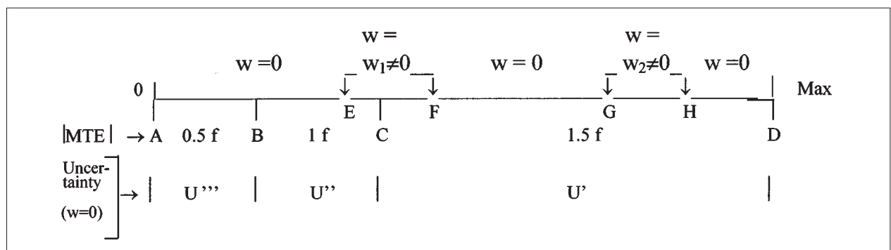
Figure 2 The weighing range 0 – Max is divided into the parts A to B, B to C and C to D. For them the values of the |\text{MTE}| 's 0.5 f, 1 f and 1.5 f and the uncertainties U''' , U'' and U' ( w = 0 ) are given respectively. However, w \neq 0 is w_1 for loads from E to F and w_2 from G to H. For these loads the values of the uncertainties U'' and U' should be corrected for w_1 and w_2 respectively, i.e., the values of U_1 (Formula B) are determined. For loads from E to C, U_1 = [U''^2 + 4w_1^2]^{1/2} and from C to F, U_1 = [U'^2 + 4w_1^2]^{1/2} . For loads from G to H, U_1 = [U'^2 + 4w_2^2]^{1/2} .
