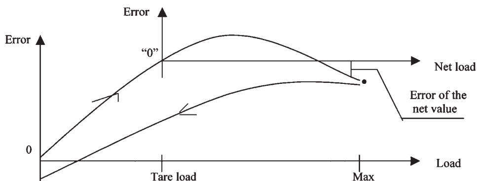
Figure 1 The ( > ) branch of the weighing curve is obtained with increasing loads and the ( < ) branch with decreasing loads. When a tare load is on the instrument a subtractive tare device (reducing the weighing range for the net loads) is used to set the indication to zero “0”.
