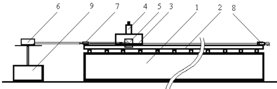
Figure 1 Scheme of comparator for long length measures
