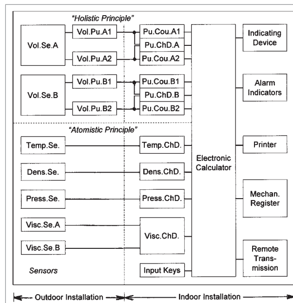
Fig. 4 Structure of the pipeline measuring system
