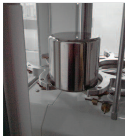
Fig. 1 Reference standard of 1 kg, Ni81
