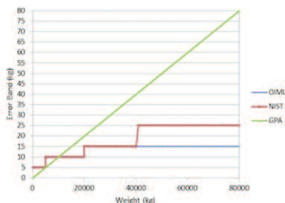
Figure 5 OIML/NIST/GPA accuracy comparison
