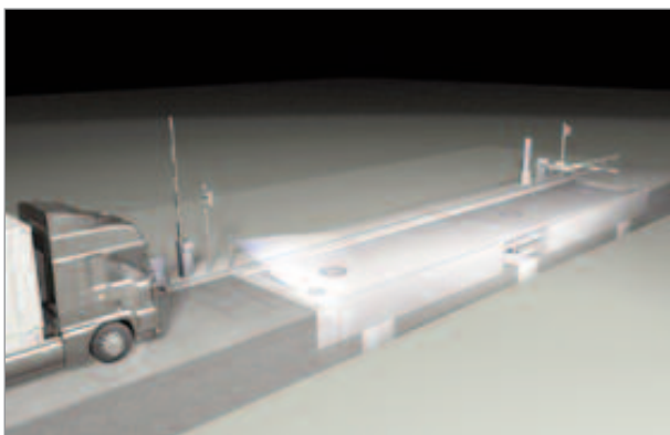
Figure 1 A pit mounted scale placed in an excavated foundation flush with the ground
