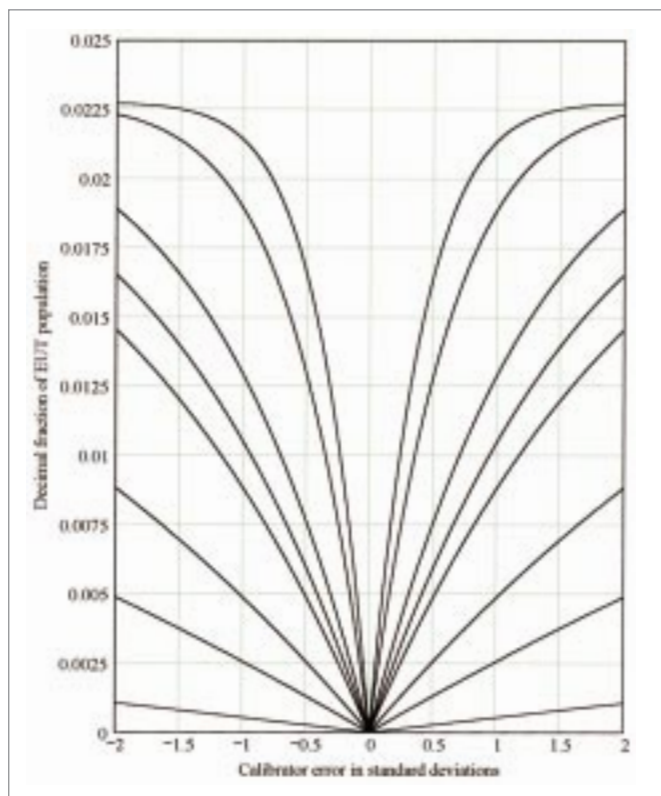
Fig. 5 Distribution of incorrect pass test decisions as a function of calibrator error for 2\sigma specifications
