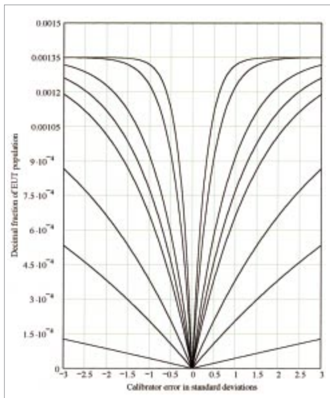
Fig. 7 Distribution of incorrect pass test decisions as a function of calibrator error for 3\sigma specifications
