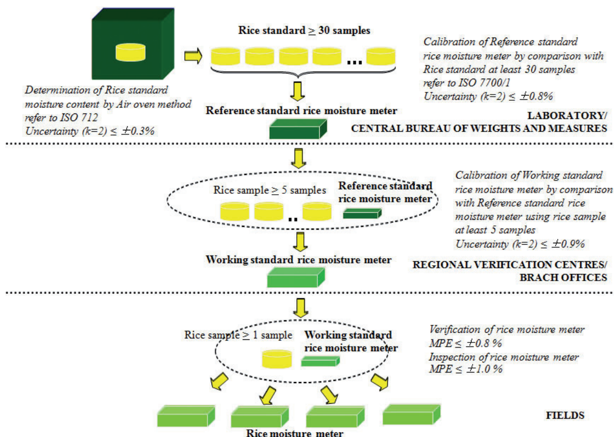
Figure 1: Traceability system of rice moisture meters
