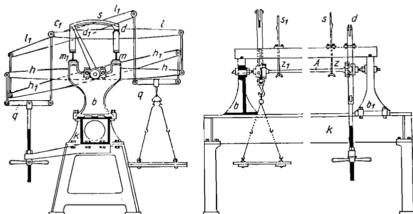
Fig. 12. Torsion tester of Wöhler.
