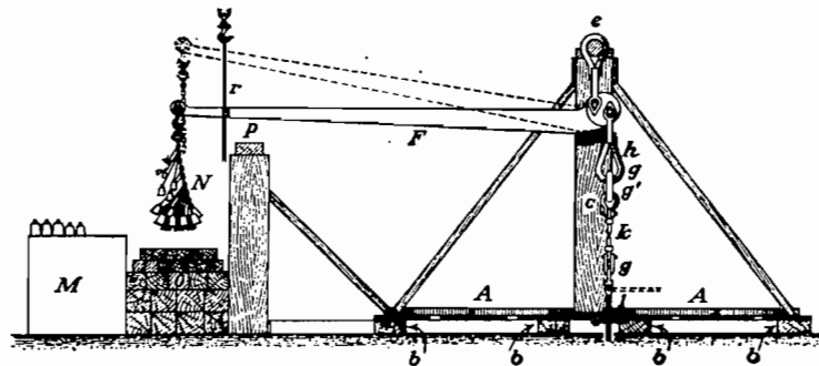
Fig. 9. An early testing machine of Kirkaldy.
