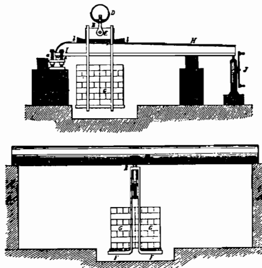
Fig. 8. Fairbairn's tube bending tester.
