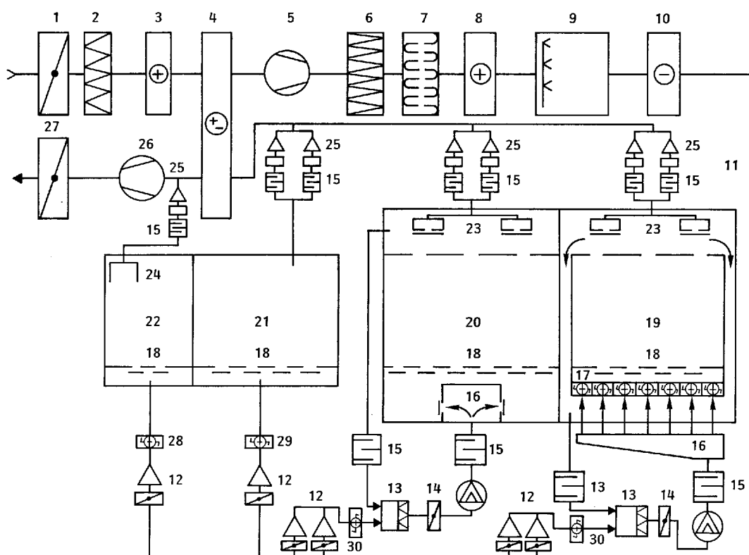
Fig. 4 : Process diagram of air-conditioning
