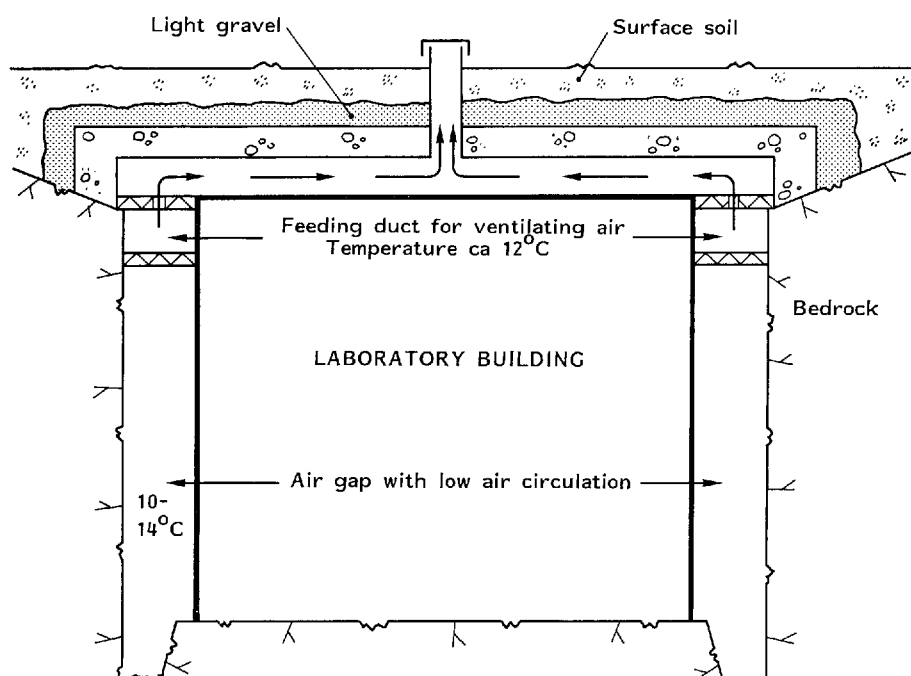
Fig. 2 : Cross-profile of laboratory
