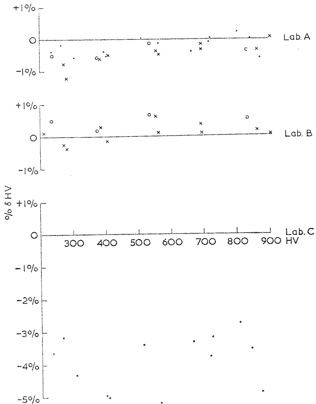
FIG.3 HV SCALES WITH RESPECT TO NPL SCALE
